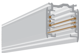
Pulse Control Track Three Circuit / Single Neutral 120V
