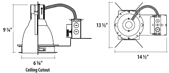
Ceiling Cutout
