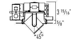
Ceiling Cut Out: 5 1/2" x 5 1/2"
