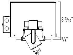
Ceiling Cut Out: 5 1/2" x 5 1/2"
